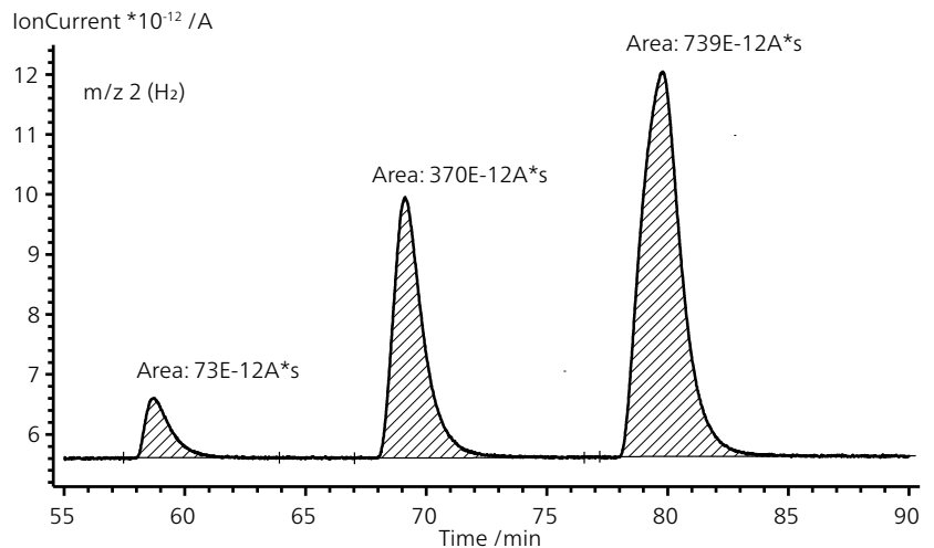
STA-MS measurement of hydrogen pulses at constant temperature
