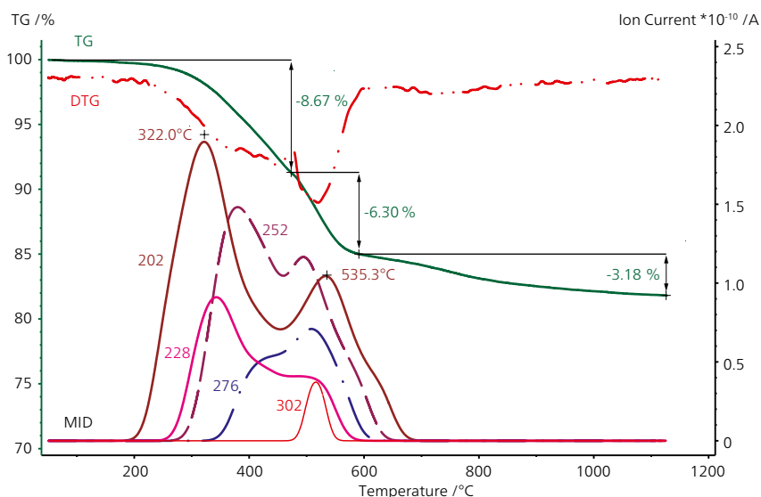
Comparison of the temperature-dependent course of mass loss and mass-loss rate of carbon pitch with ion current curves of typical mass numbers of aromatic compounds
