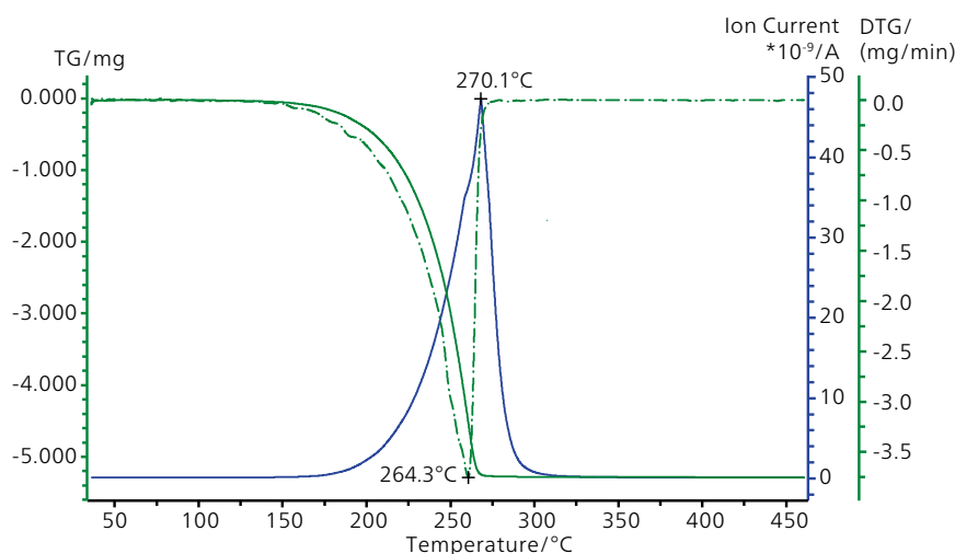
Temperature-dependent mass loss, mass loss rate and total ion current for evaporation of heptadecane
