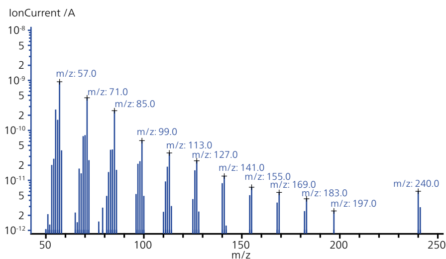
Significant fragmentation pattern of heptadecane at 250°C
