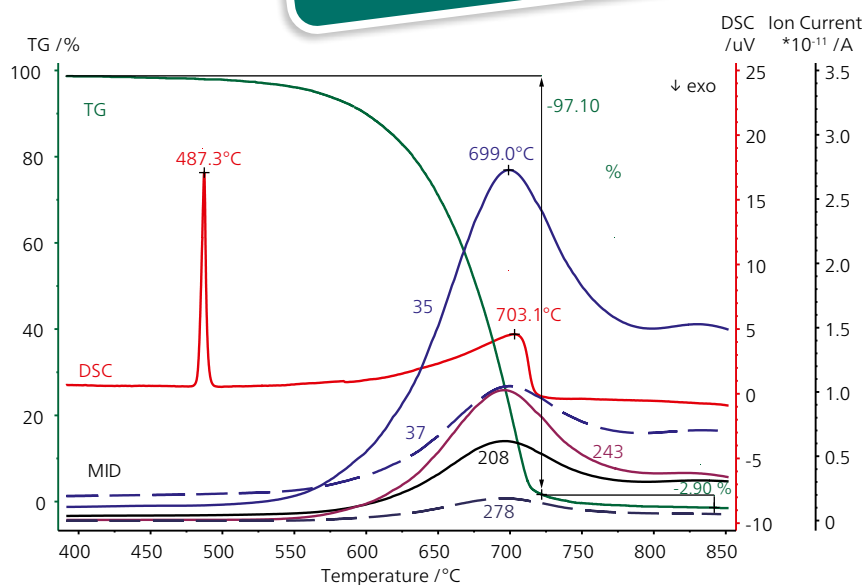
Comparison of the mass loss and DSC curve of \text{PbCl}_2 with the ion current curves of the fragment ions
