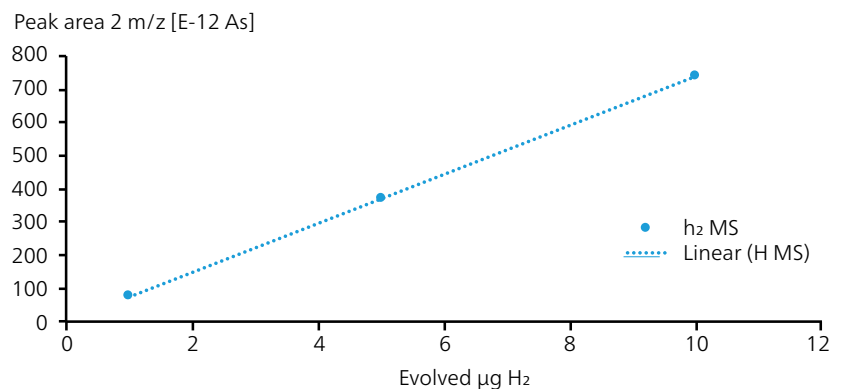
Presentation of the linear relationship between pulse area and the amount of hydrogen gas (H 2 )
