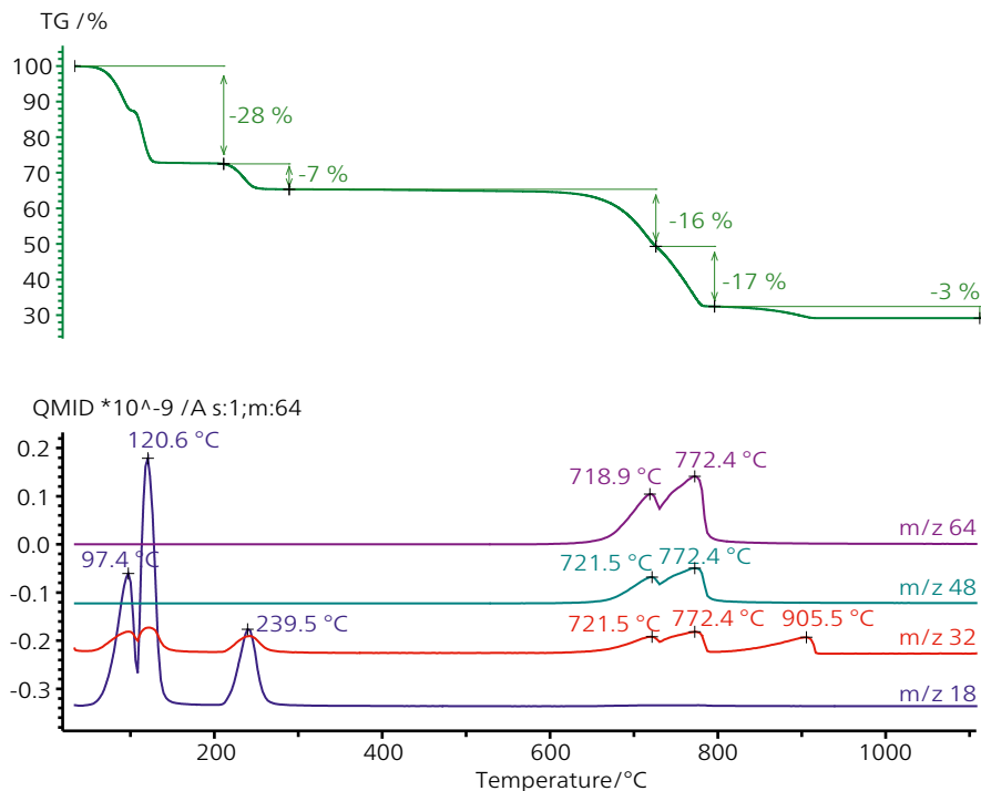
Thermogram of blue vitriol in combination with the ion current curves of m/z 18, 32, 48 and 64
