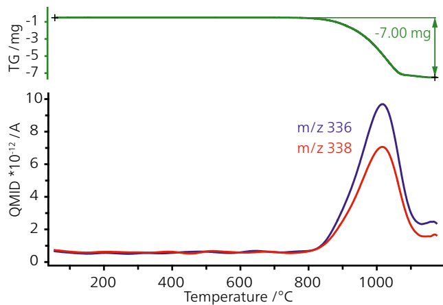
Correlation of the ion current (QMID) of fragment masses m/z 332 to 338 with the mass-loss curve (TGA) of PbTe
