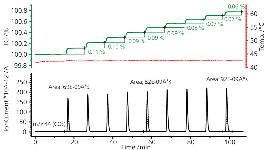
Isothermal treatment of CaO (177.8 mg) on a Pt grid sample carrier at 43°C in a dry argon atmosphere with pulses of 250 µl of CO 2
