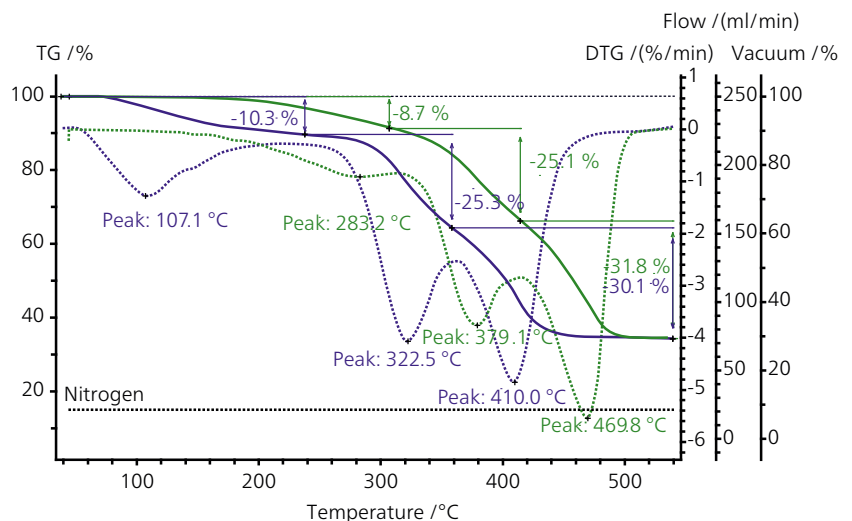
TGA measurements were taken on a bicycle tire casing at a heating rate of 10 K/min. Measurements were taken under nitrogen (green curves) and under vacuum (blue curves). TGA curves are shown as solid lines and DTG curves are shown as dashed lines
